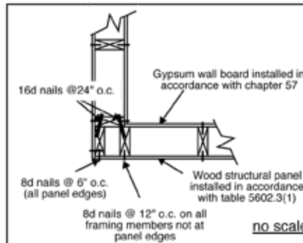
FIGURE 5602.10.5 EXTERIOR CORNER FRAMING
